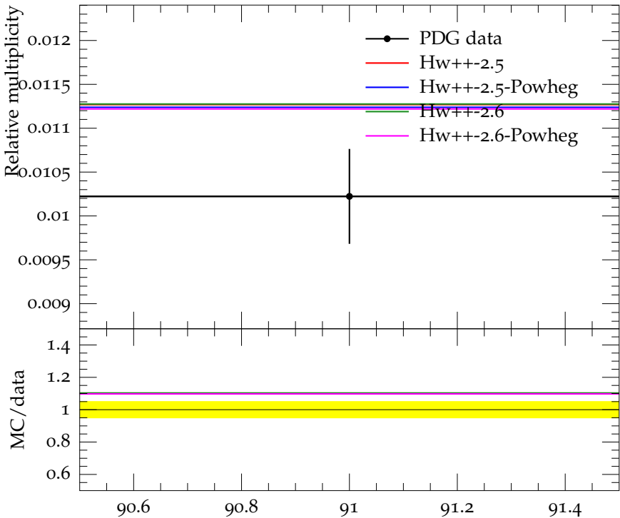
Ratio (w.r.t. \pi^\pm ) of mean \Sigma^\pm multiplicity
