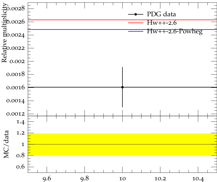
Ratio (w.r.t. \pi^\pm ) of mean \Sigma^\pm(1385) multiplicity
