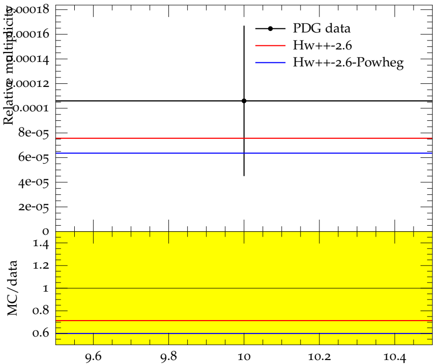
Ratio (w.r.t. \pi^\pm ) of mean \Omega^- multiplicity
