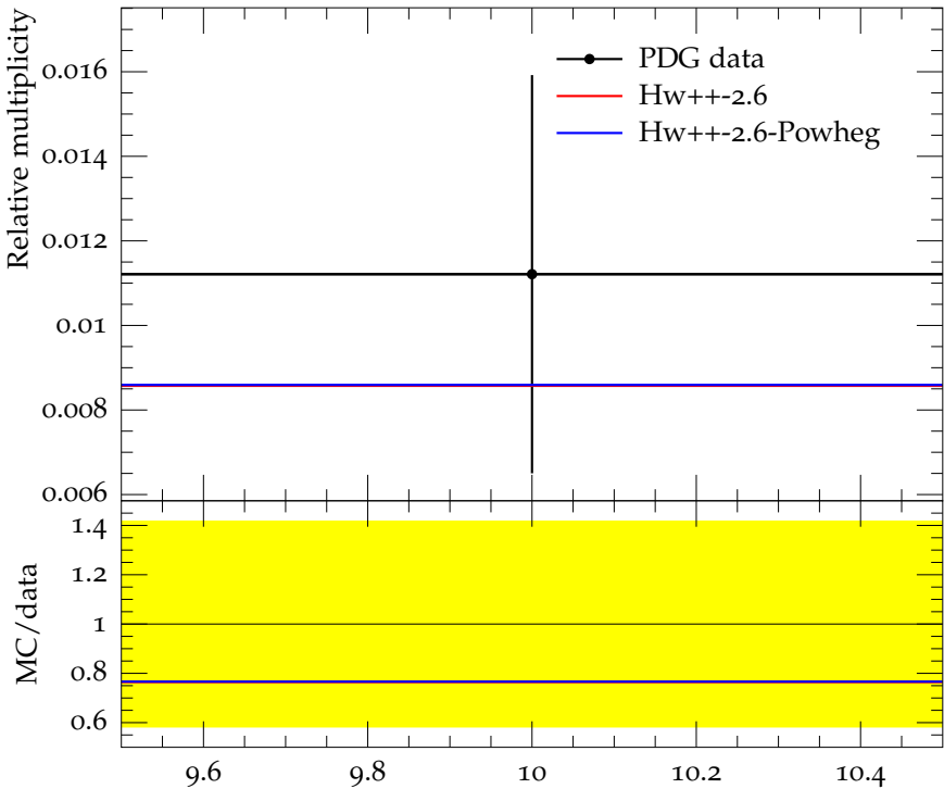
Ratio (w.r.t. \pi^\pm ) of mean \Lambda_c^+ multiplicity
