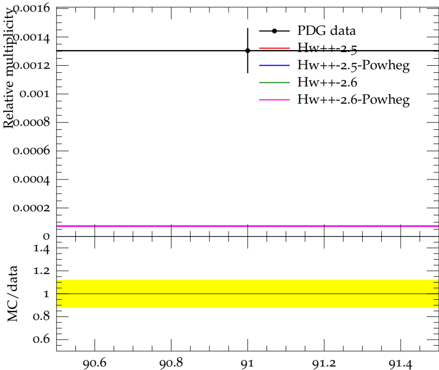
Ratio (w.r.t. \pi^\pm ) of mean \Lambda(1520) multiplicity
