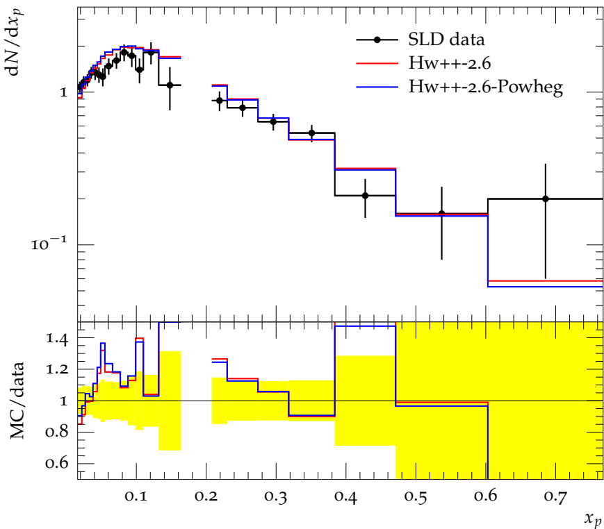
K^+ scaled momentum, ratio b to uds events
