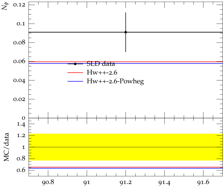
Multiplicity of \phi in ( uds ) events
