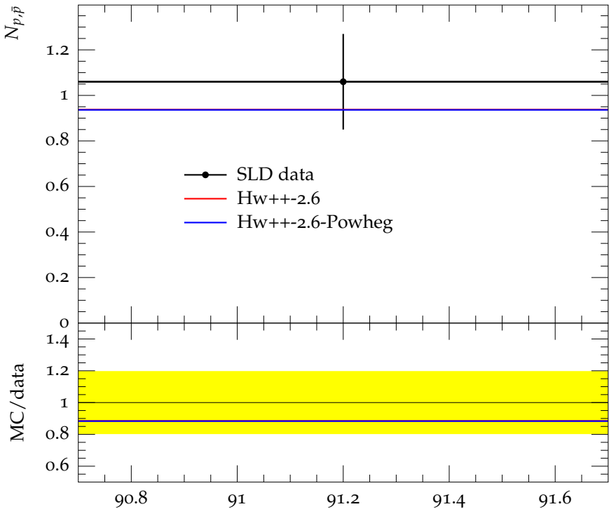
Multiplicity of p, \bar{p} in c events
