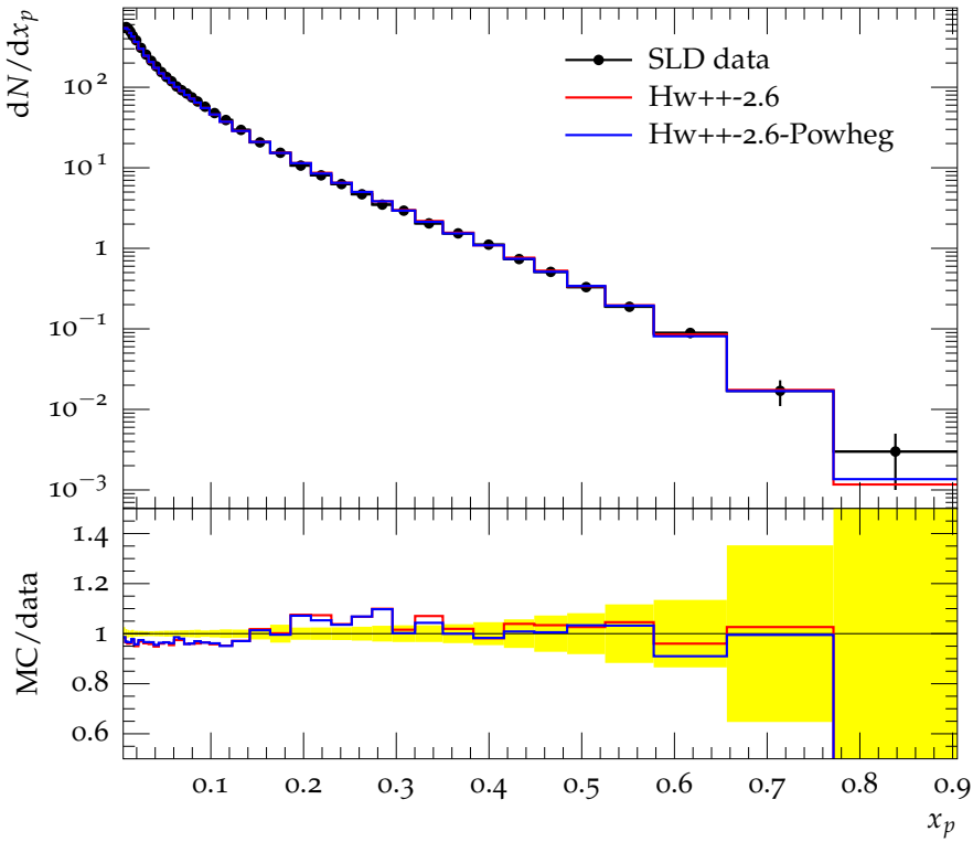
Charged particle scaled Momentum, b events
