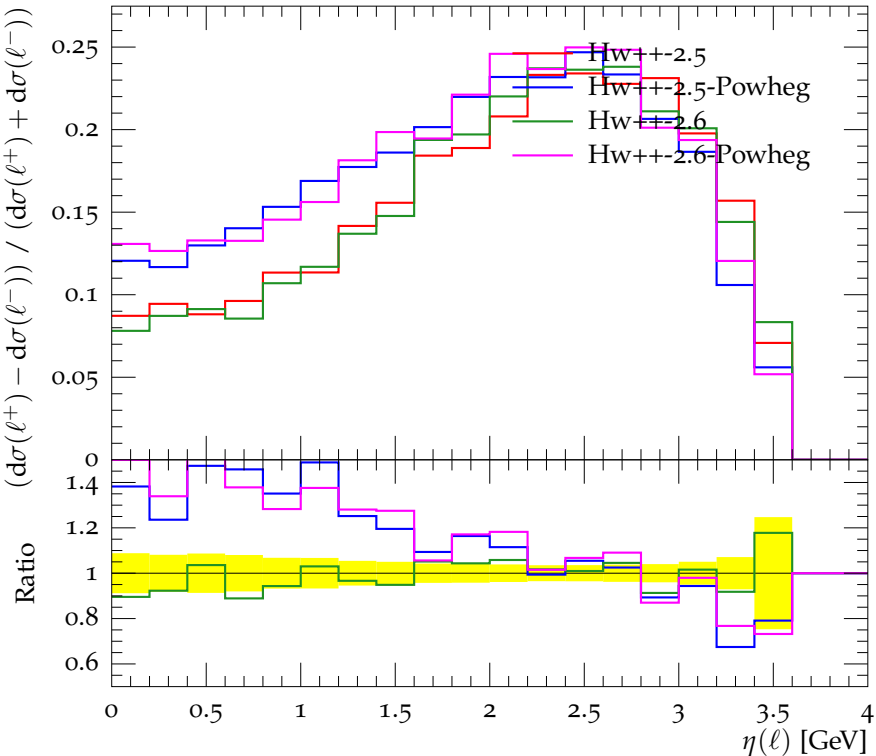
Charge asymmetry vs. \eta(\ell)
