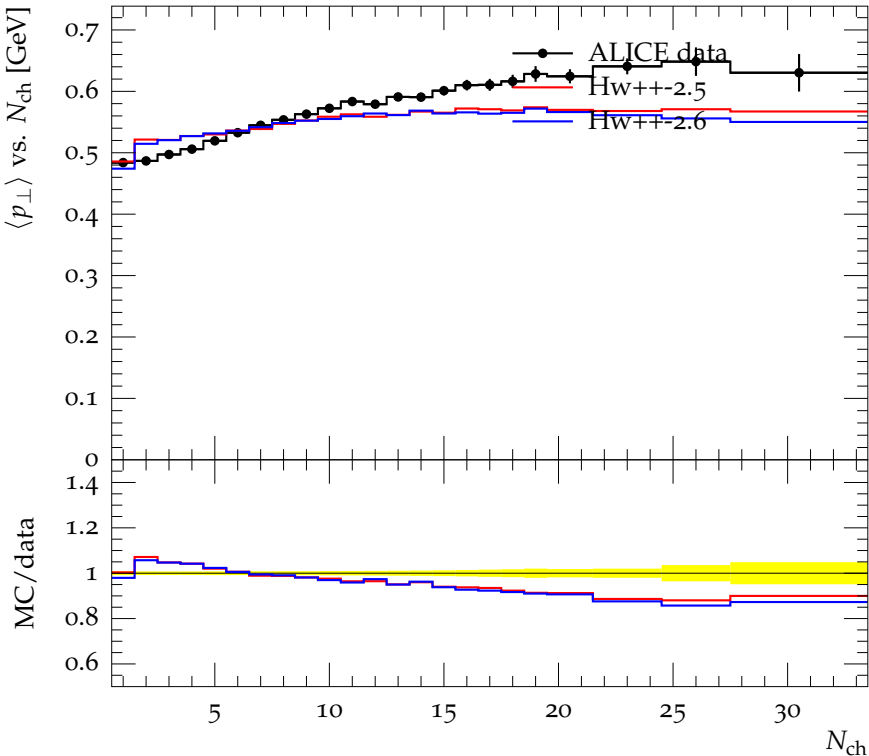
Avg. transv. momentum vs. N_{\text{ch}} ( 0.15 \leq p_{\perp} \leq 4 GeV)
