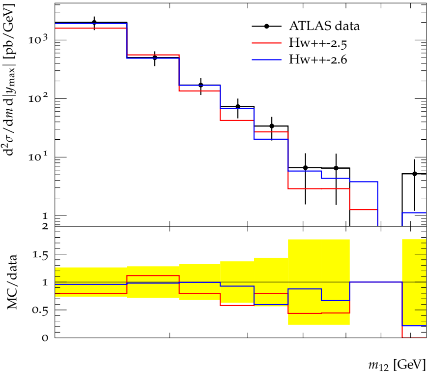
Dijet mass spectrum for |y_{\max}| < 0.3 , anti-KT, R = 0.4 .
