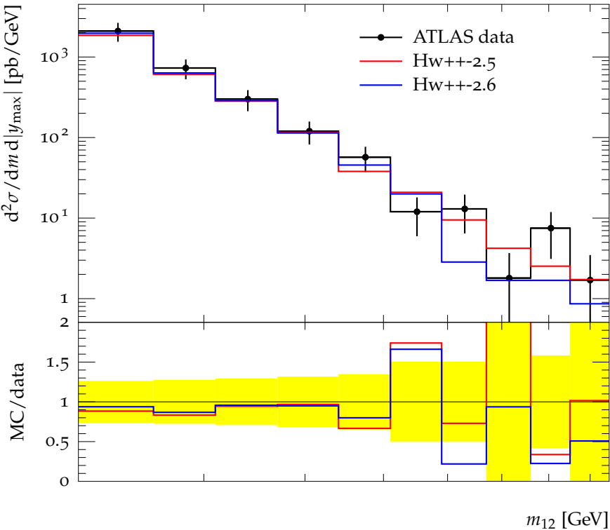
Dijet mass spectrum for 0.8 < |y_{\max}| < 1.2 . anti-KT, R = 0.4 .
