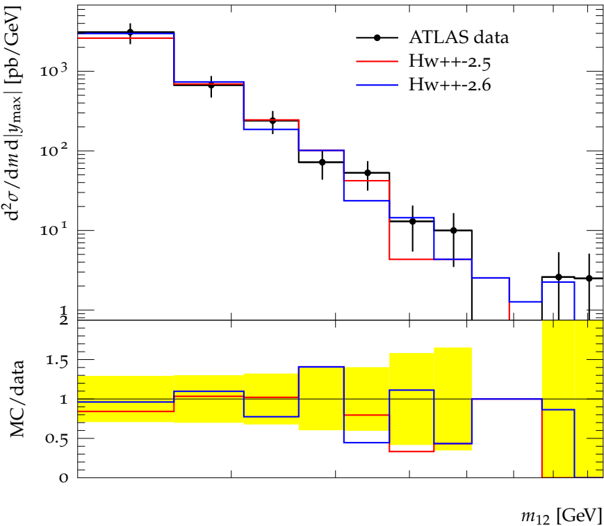
Dijet mass spectrum for |y_{\max}| < 0.3 , anti-KT, R = 0.6 .
