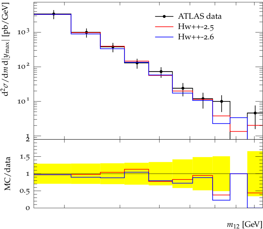
Dijet mass spectrum for 0.3 < |y_{\max}| < 0.8 . anti-KT, R = 0.6 .
