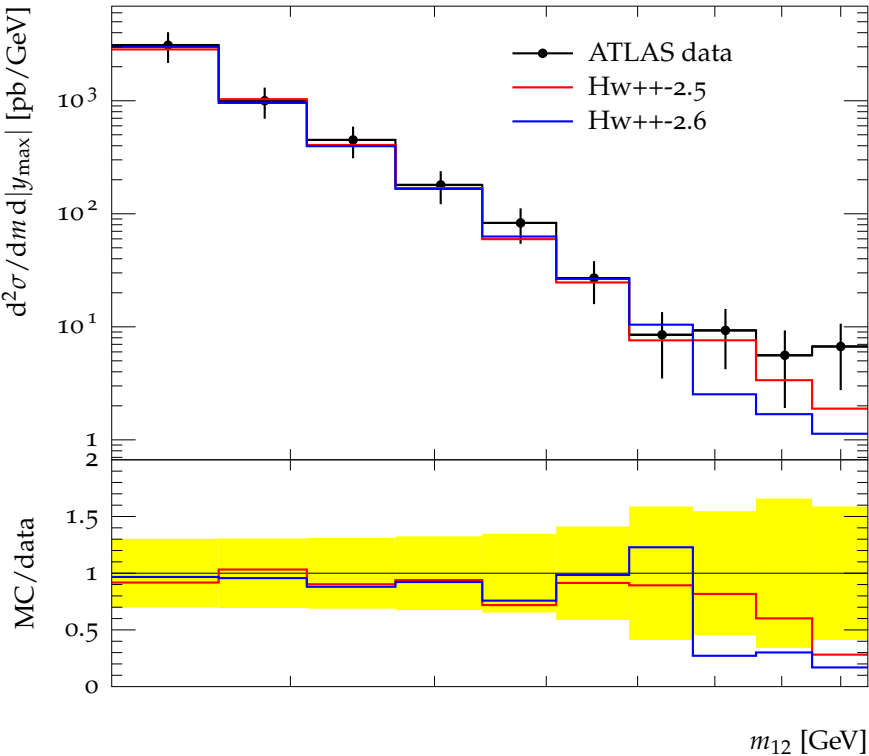
Dijet mass spectrum for 0.8 < |y_{\max}| < 1.2 . anti-KT, R = 0.6 .
