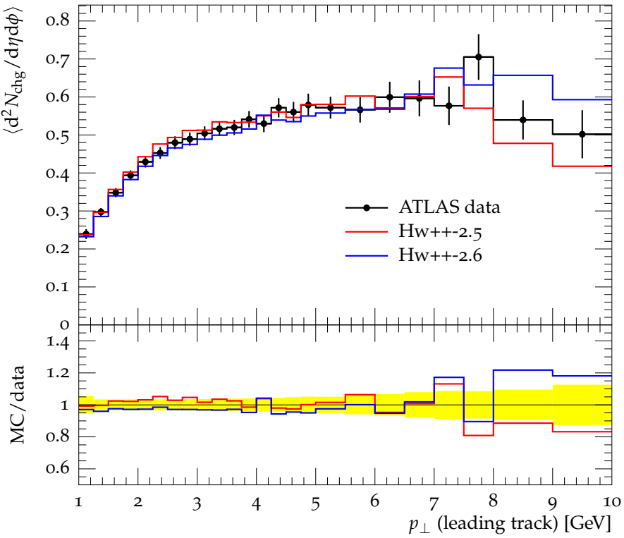
Toward N_{\text{chg}} density vs. p_{\perp}^{\text{trk1}} , \sqrt{s} = 900 GeV
