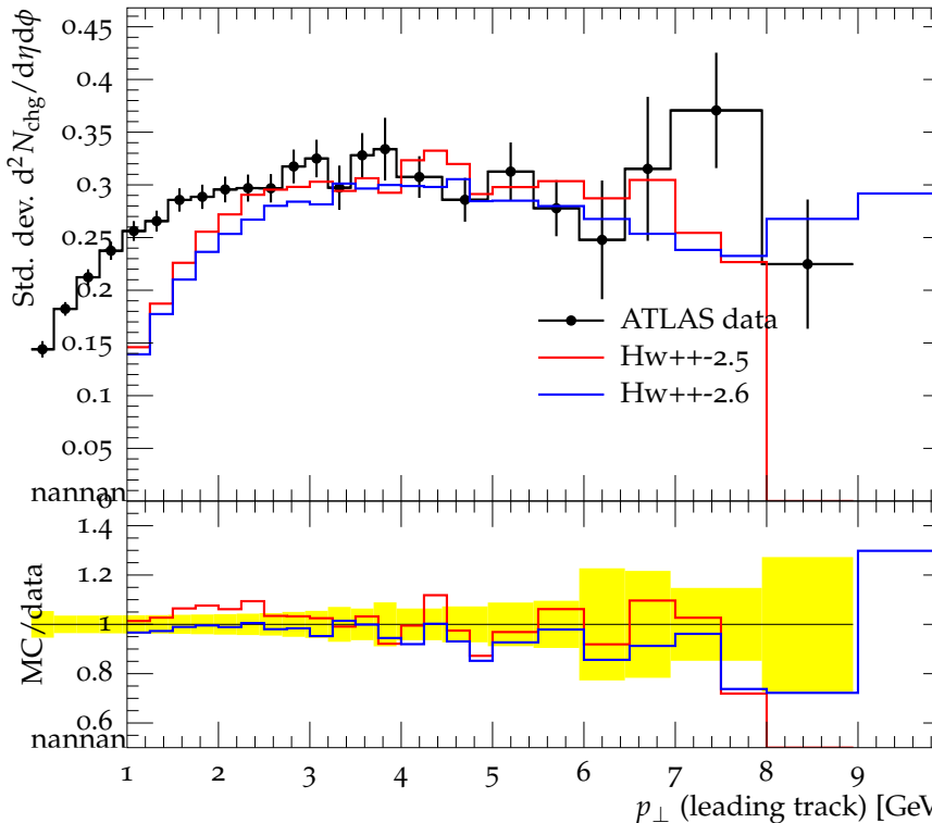
Std. dev. Transverse N_{\text{chg}} density vs. p_{\perp}^{\text{trk1}} , \sqrt{s} = 900 GeV
