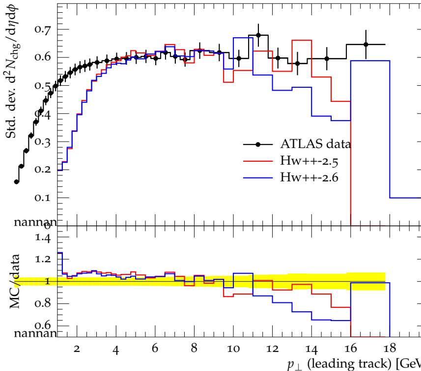
Std. dev. Transverse N_{\text{chg}} density vs. p_{\perp}^{\text{trk1}} , \sqrt{s} = 7 TeV
