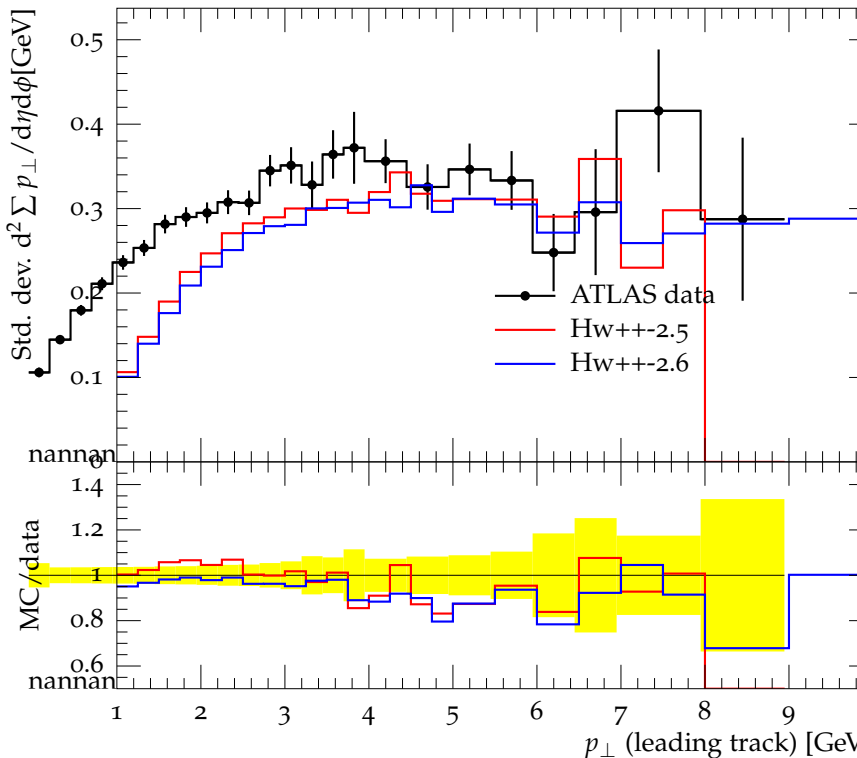
Std. dev. Transverse \Sigma p_{\perp} density vs. p_{\perp}^{\text{trk1}} , \sqrt{s} = 900 GeV
