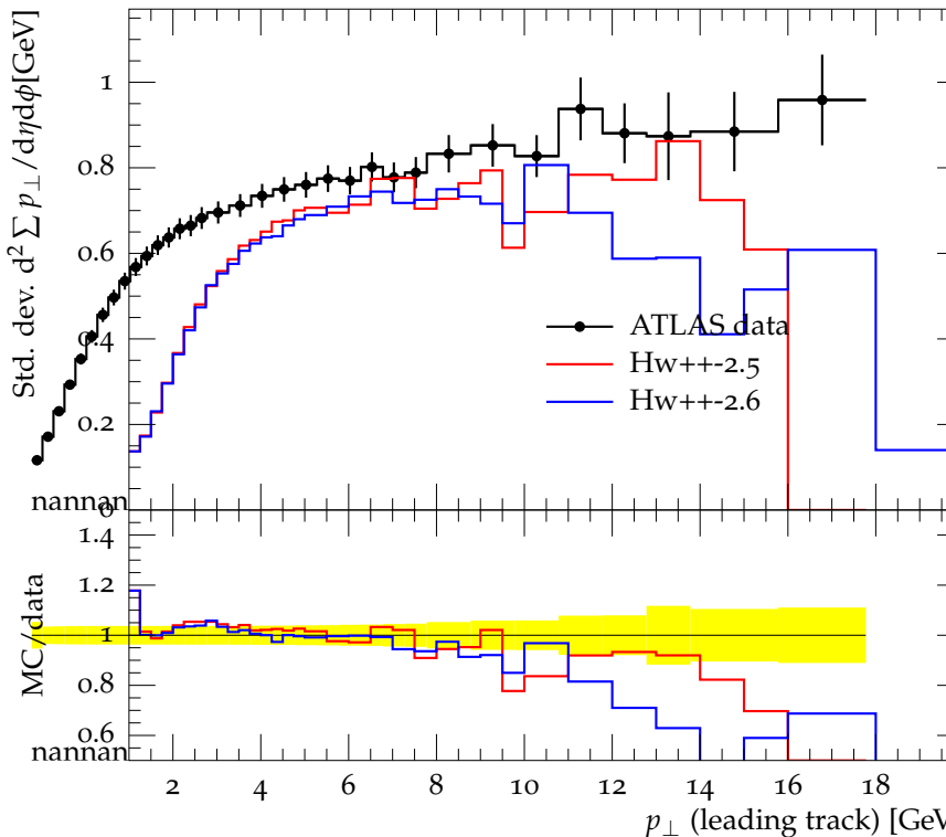
Std. dev. Transverse \Sigma p_{\perp} density vs. p_{\perp}^{\text{trk1}} , \sqrt{s} = 7 TeV
