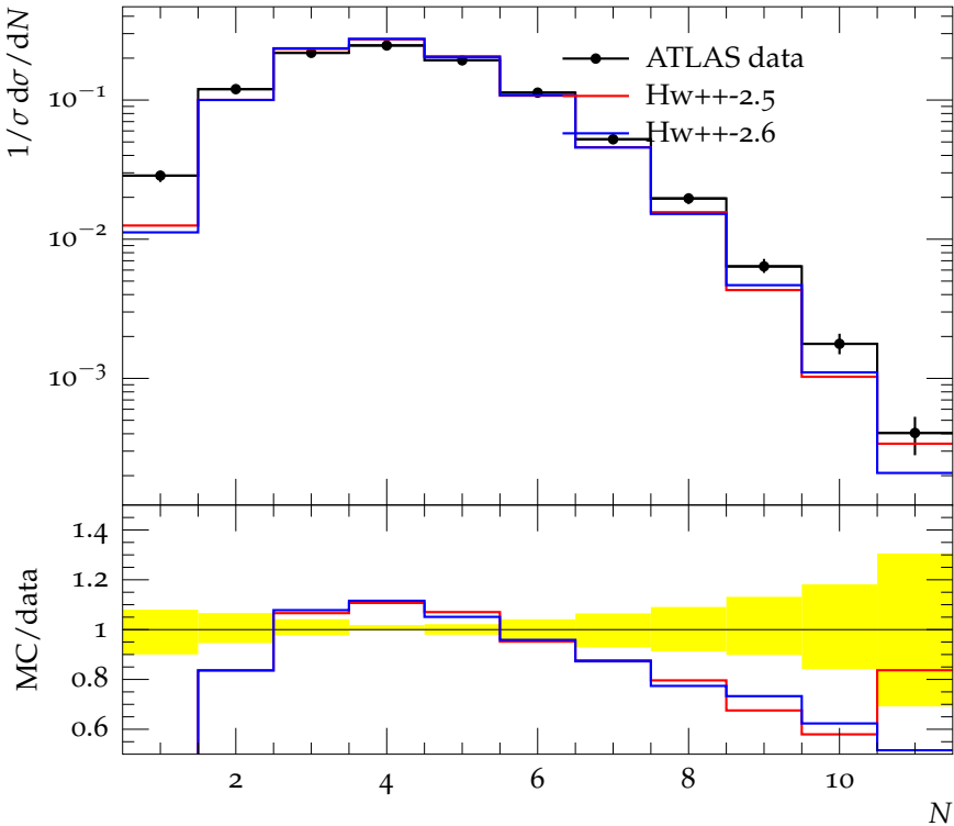
Charged jet multiplicity (anti- k_t , R = 0.4 , y 0.0-1.9, p_\perp 6.0-10.0)
