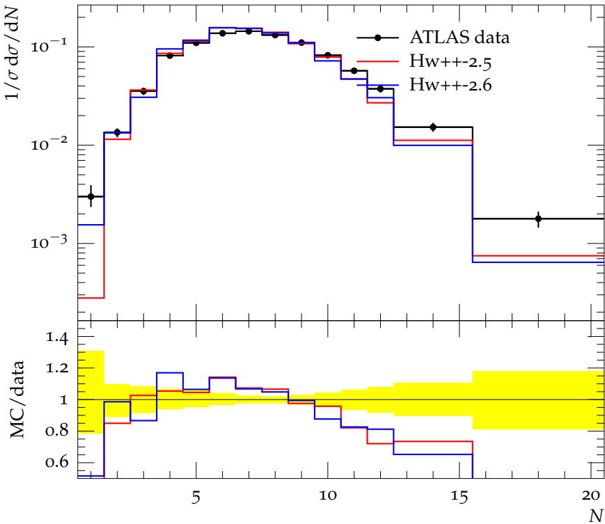
Charged jet multiplicity (anti- k_t , R = 0.4 , y 0.0-1.9, p_\perp 24.0-40.0)
