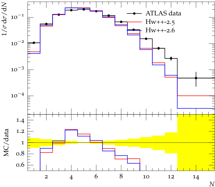
Charged jet multiplicity (anti- k_t , R = 0.4 , y 0.0-0.5, p_\perp 10.0-15.0)
