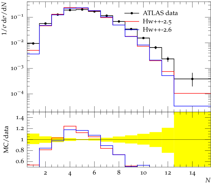
Charged jet multiplicity (anti- k_t , R = 0.4 , y 0.5-1.0, p_\perp 10.0-15.0)
