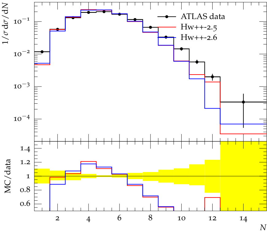
Charged jet multiplicity (anti- k_t , R = 0.4 , y 1.0-1.5, p_\perp 10.0-15.0)
