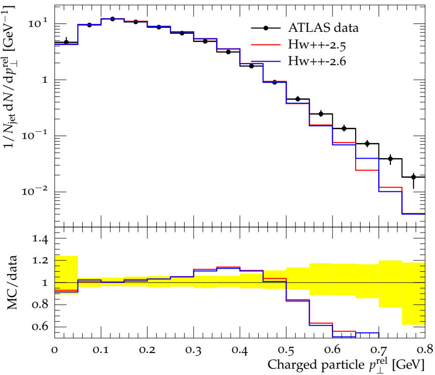
Charged jet p_{\perp}^{\text{rel}} (anti- k_t , R = 0.4 , y 1.5-1.9, p_{\perp} 4.0-6.0)
