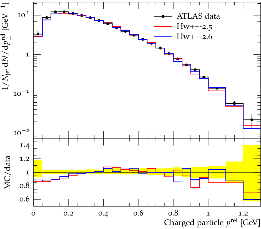
Charged jet p_{\perp}^{\text{rel}} (anti- k_t , R = 0.4 , y 1.5-1.9, p_{\perp} 10.0-15.0)
