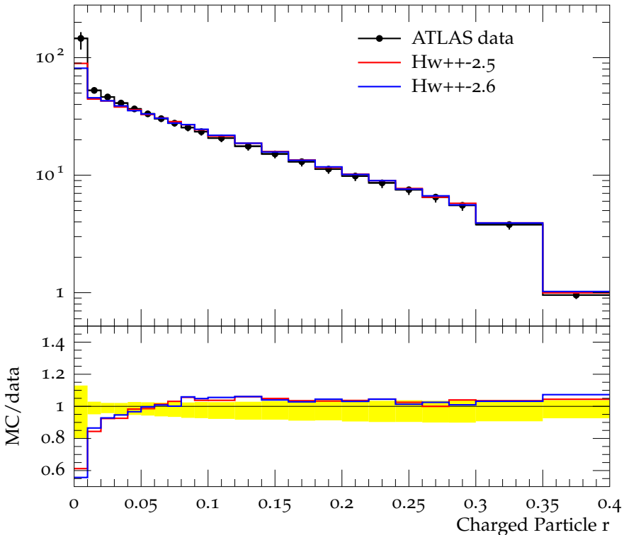
Charged jet \rho_{\text{ch}}(r) (anti- k_t , R = 0.4 , y 0.0-1.9, p_{\perp} 6.0-10.0)
