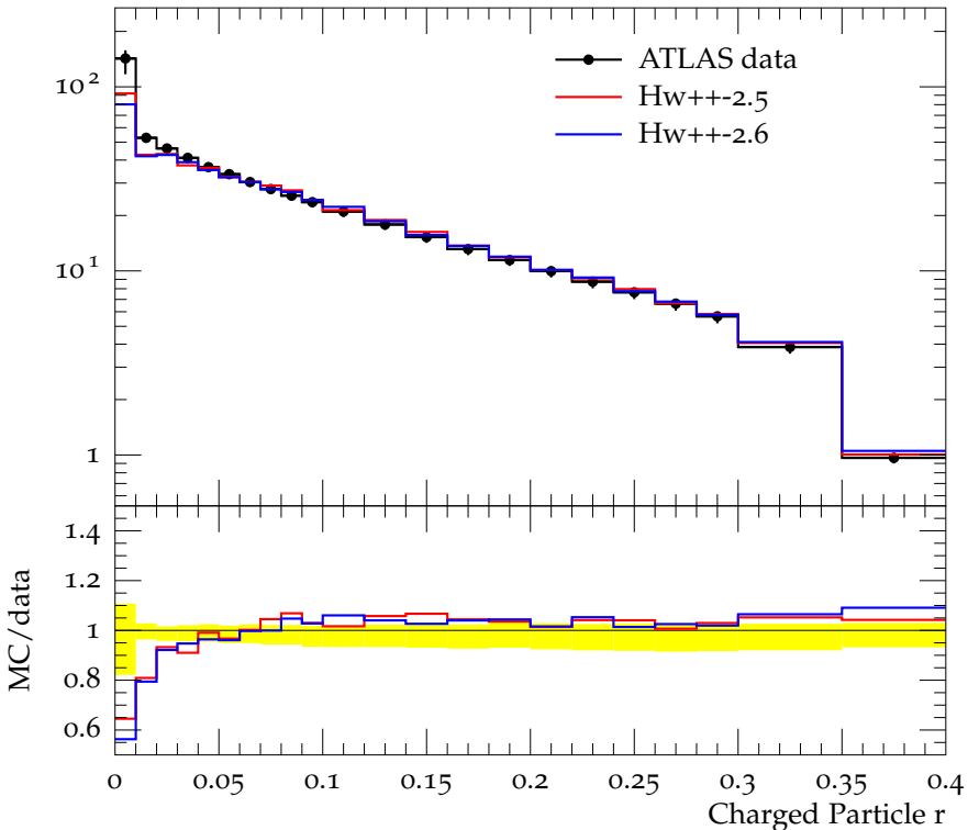
Charged jet \rho_{\text{ch}}(r) (anti- k_t , R = 0.4 , y 0.0-0.5, p_{\perp} 6.0-10.0)
