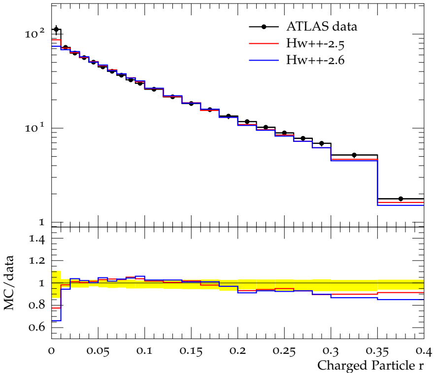
Charged jet \rho_{\text{ch}}(r) (anti- k_t , R = 0.4 , y 0.0-0.5, p_{\perp} 10.0-15.0)
