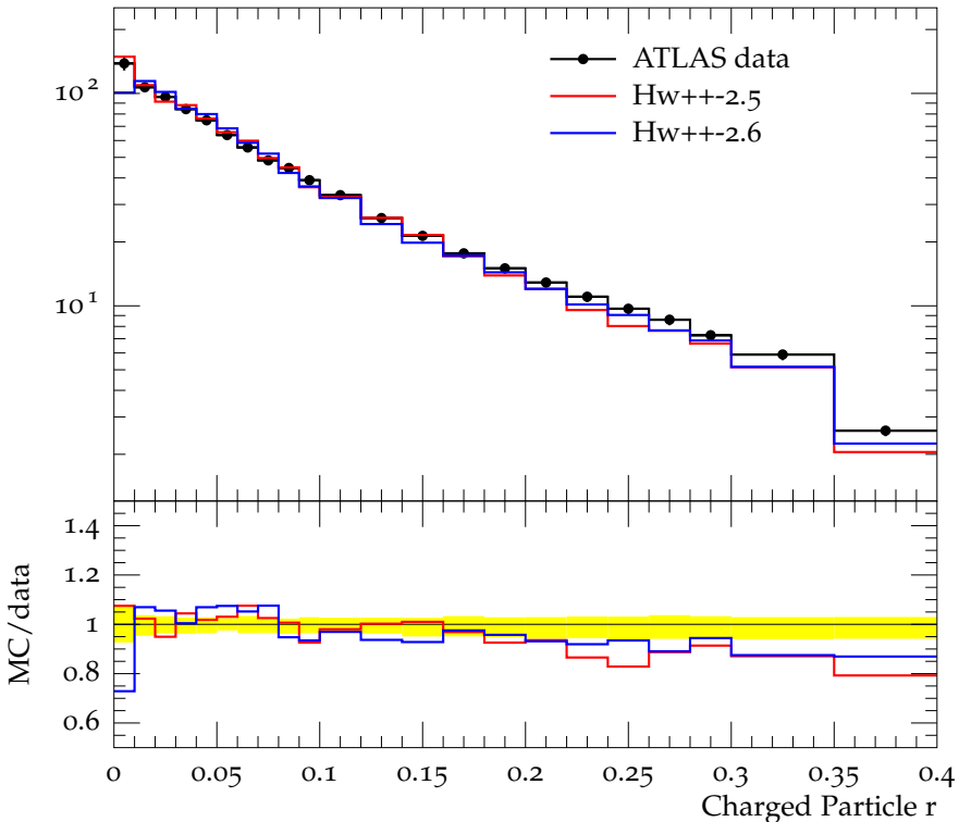
Charged jet \rho_{\text{ch}}(r) (anti- k_t , R = 0.4 , y 0.0-0.5, p_{\perp} 15.0-24.0)
