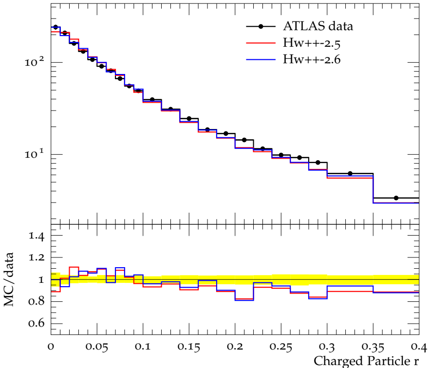
Charged jet \rho_{\text{ch}}(r) (anti- k_t , R = 0.4 , y 0.0-0.5, p_{\perp} 24.0-40.0)
