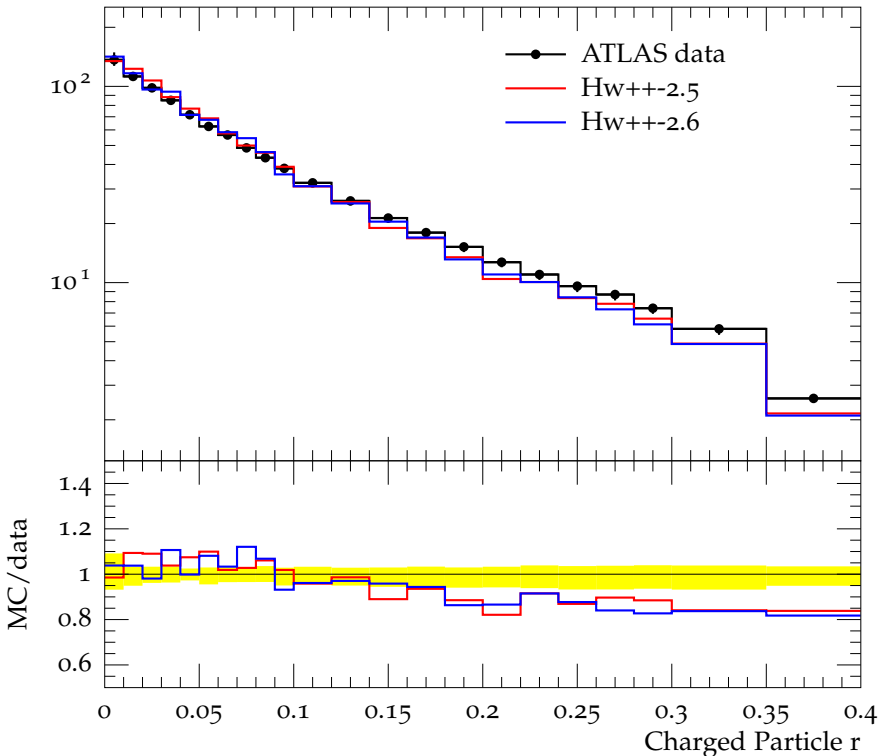
Charged jet \rho_{\text{ch}}(r) (anti- k_t , R = 0.4 , y 0.5-1.0, p_{\perp} 15.0-24.0)
