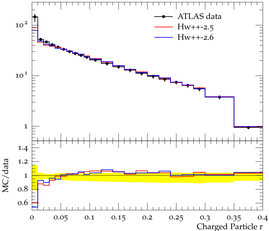
Charged jet \rho_{\text{ch}}(r) (anti- k_t , R = 0.4 , y 1.0-1.5, p_{\perp} 6.0-10.0)
