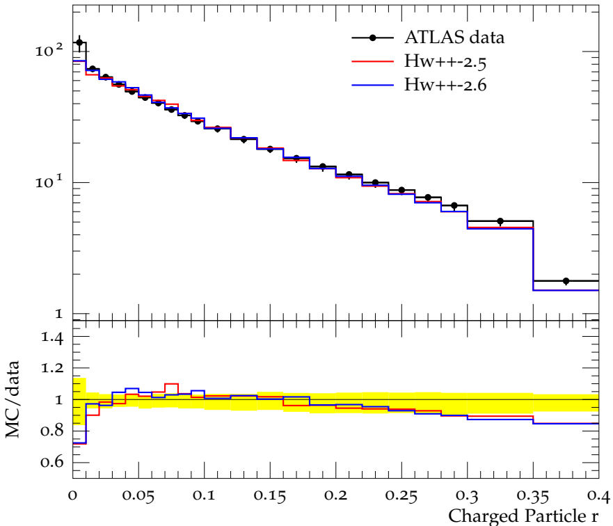
Charged jet \rho_{\text{ch}}(r) (anti- k_t , R = 0.4 , y 1.0-1.5, p_{\perp} 10.0-15.0)
