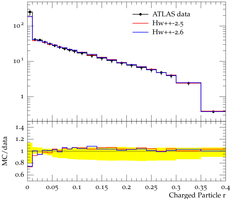
Charged jet \rho_{\text{ch}}(r) (anti- k_t , R = 0.4 , y 1.5-1.9, p_{\perp} 4.0-6.0)
