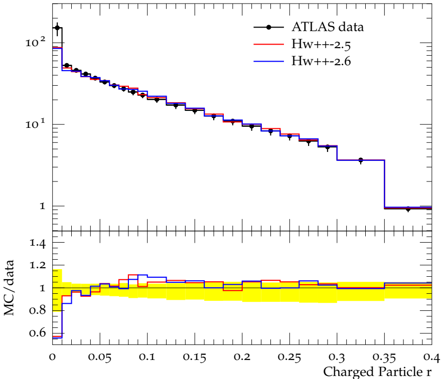
Charged jet \rho_{\text{ch}}(r) (anti- k_t , R = 0.4 , y 1.5-1.9, p_{\perp} 6.0-10.0)
