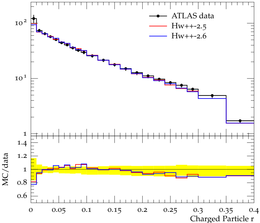
Charged jet \rho_{\text{ch}}(r) (anti- k_t , R = 0.4 , y 1.5-1.9, p_{\perp} 10.0-15.0)
