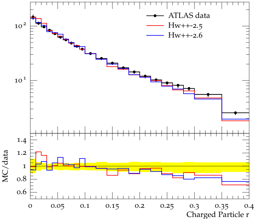
Charged jet \rho_{\text{ch}}(r) (anti- k_t , R = 0.4 , y 1.5-1.9, p_{\perp} 15.0-24.0)
