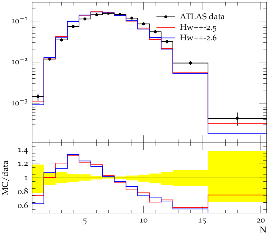
Charged jet multiplicity (anti- k_t , R = 0.6 , y 0.5-1.0, p_\perp 10.0-15.0)
