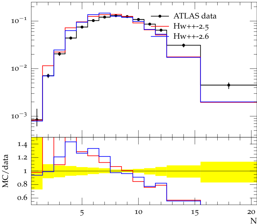
Charged jet multiplicity (anti- k_t , R = 0.6 , y 0.5-1.0, p_\perp 15.0-24.0)
