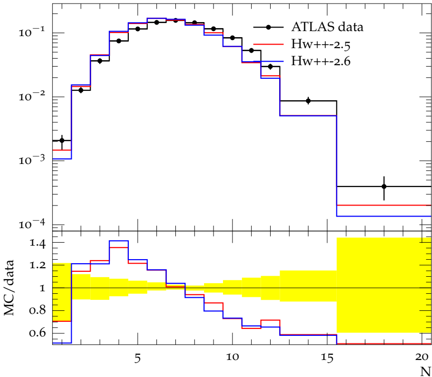
Charged jet multiplicity (anti- k_t , R = 0.6 , y 1.0-1.5, p_\perp 10.0-15.0)
