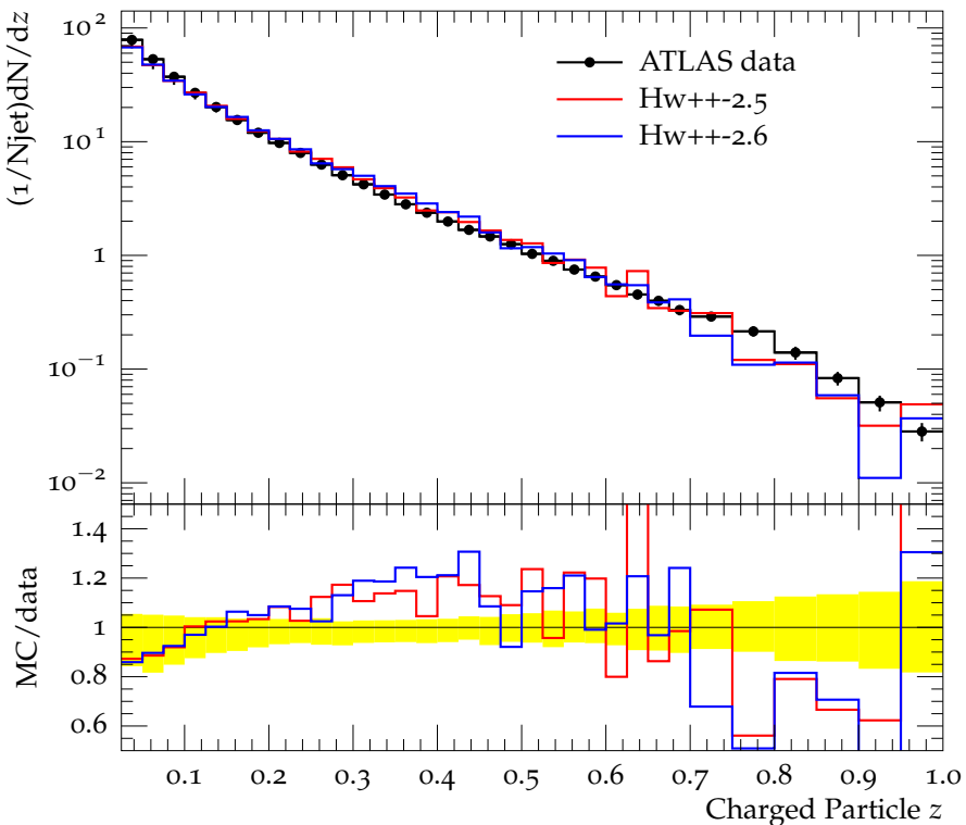
Charged jet z (anti- k_t , R = 0.6 , y 1.0-1.5, p_\perp 15.0-24.0)
