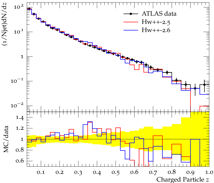
Charged jet z (anti- k_t , R = 0.6 , y 1.5-1.9, p_\perp 24.0-40.0)
