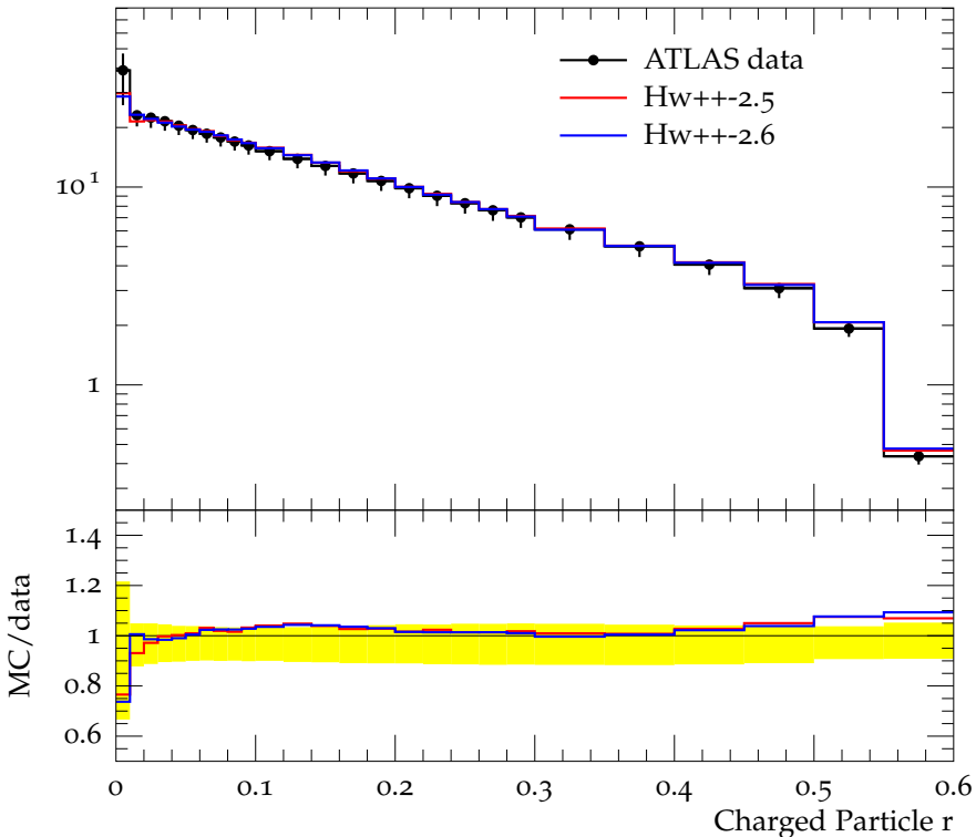
Charged jet \rho_{\text{ch}}(r) (anti- k_t , R = 0.6 , y 0.0-1.9, p_{\perp} 6.0-10.0)
