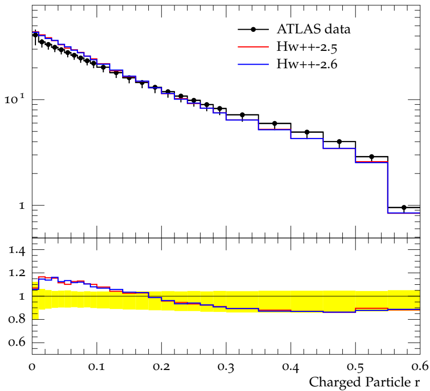
Charged jet \rho_{\text{ch}}(r) (anti- k_t , R = 0.6 , y 0.0-1.9, p_{\perp} 10.0-15.0)
