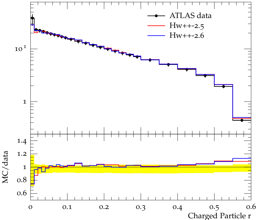
Charged jet \rho_{\text{ch}}(r) (anti- k_t , R = 0.6 , y 0.0-0.5, p_{\perp} 6.0-10.0)
