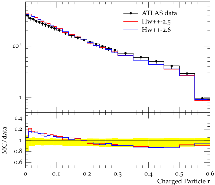
Charged jet \rho_{\text{ch}}(r) (anti- k_t , R = 0.6 , y 0.0-0.5, p_{\perp} 10.0-15.0)
