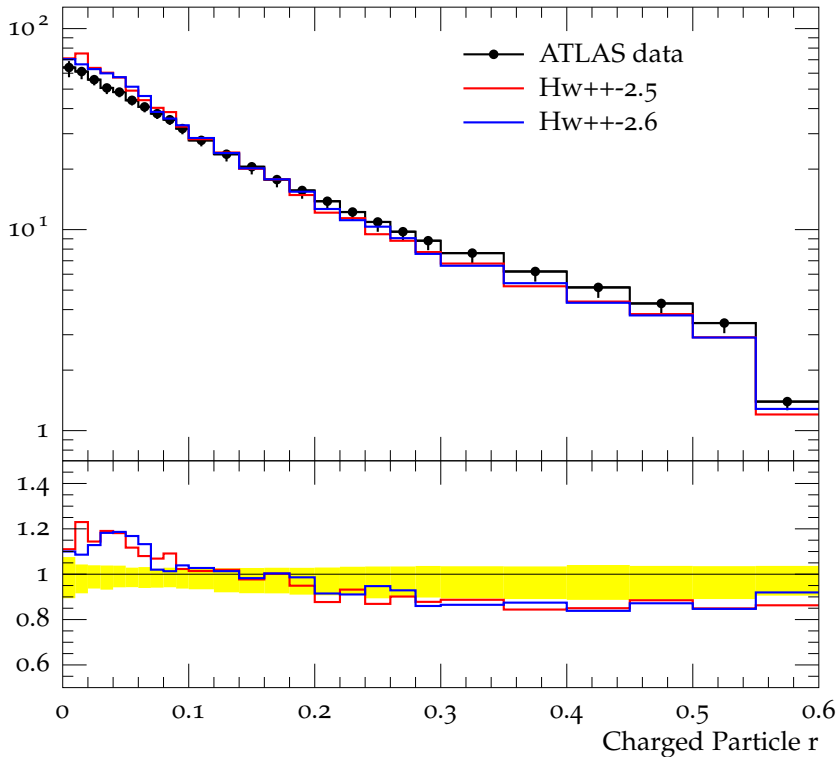
Charged jet \rho_{\text{ch}}(r) (anti- k_t , R = 0.6 , y 0.0-0.5, p_{\perp} 15.0-24.0)
